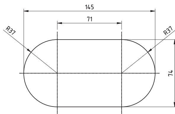
CUTTING HOLE
